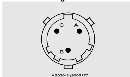
Fig. 2 Connector assignment AS-020
