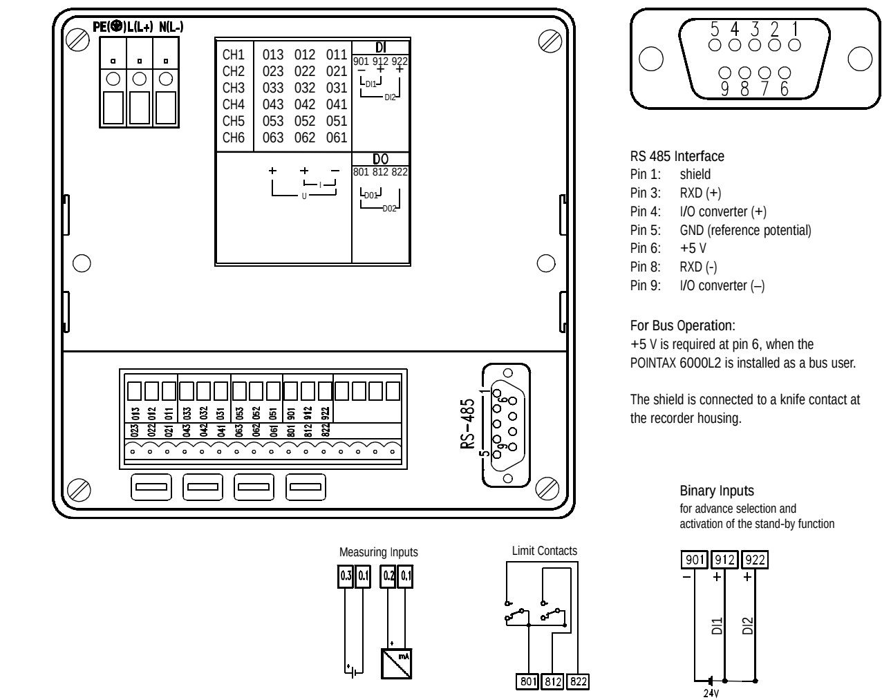
Wiring Diagram
