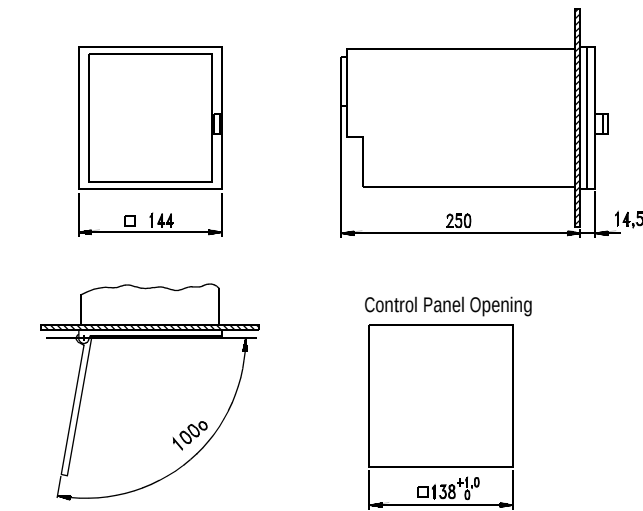
Dimensional Drawing (dimensions in mm)
