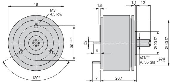
Fig. 6. KINAX 2W2 with special drive shaft at front and at rear. Front: dia. 1/4", length 12 mm [0.472"]. Rear: dia. 2 mm, length 6 mm [0.236"].
