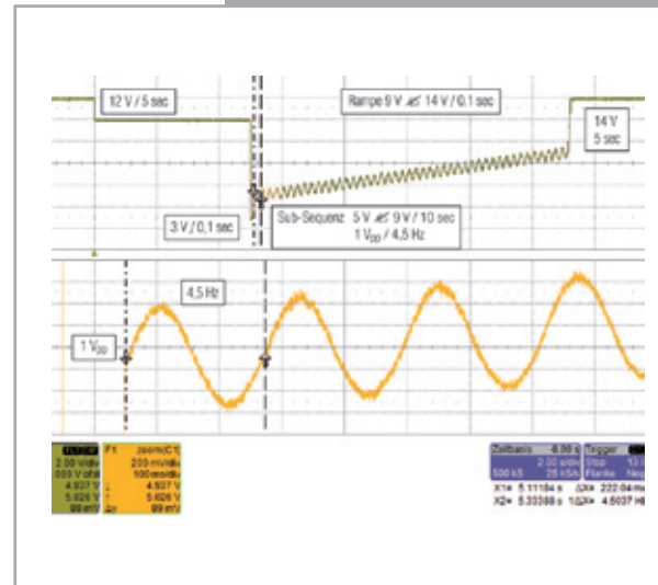
Generation of a starter motor characteristic curve
