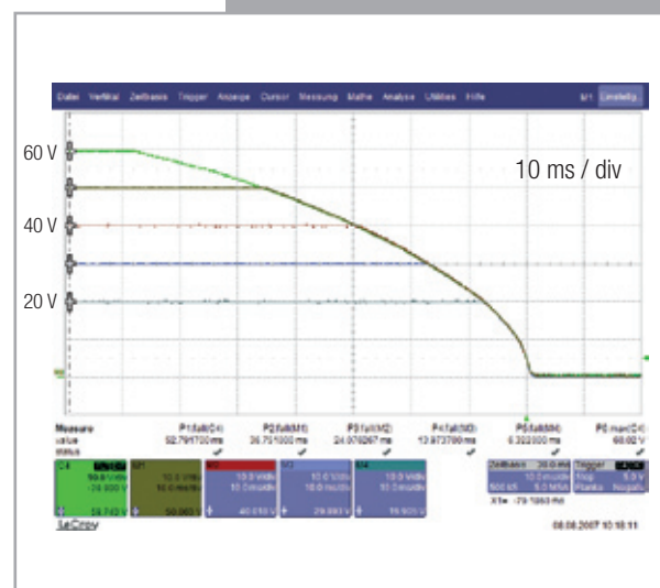
Descending time of pre-set nominal power
