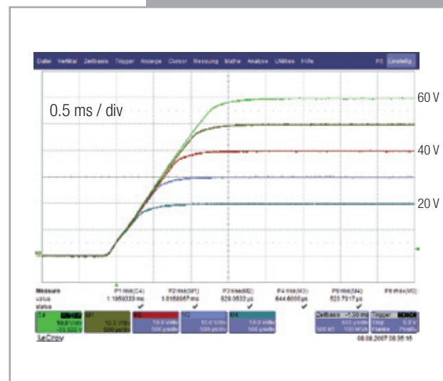
Rise time of pre-set nominal power
