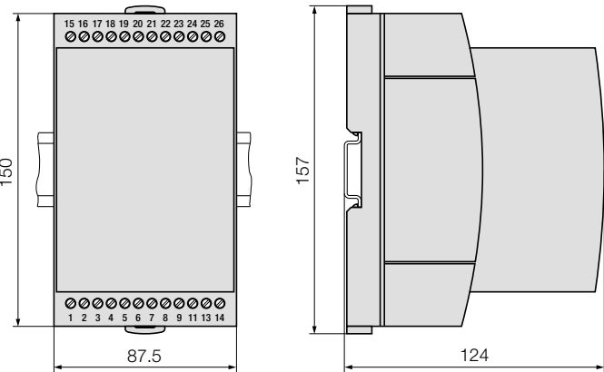
Fig. 4. SINEAX DME 400 in housing T24 clipped onto a top-hat rail (35 × 15 mm or 35 × 7.5 mm, acc. to EN 50 022).
