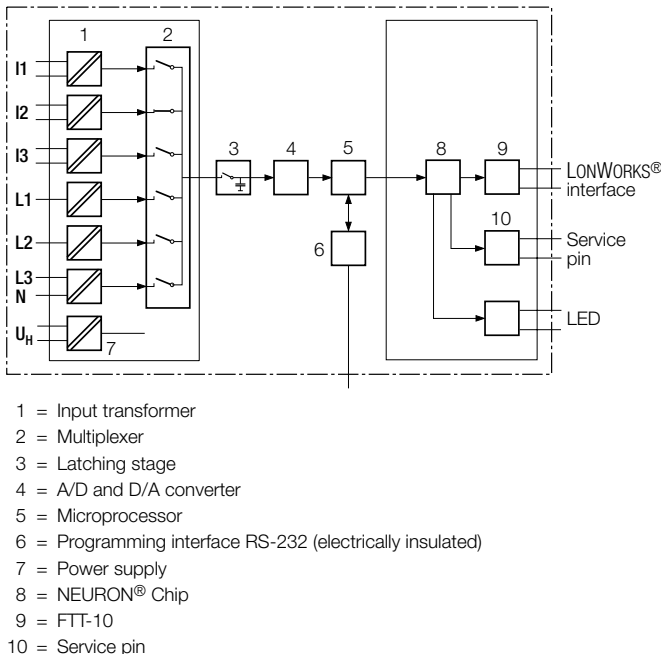
Fig. 2. Block diagram.
